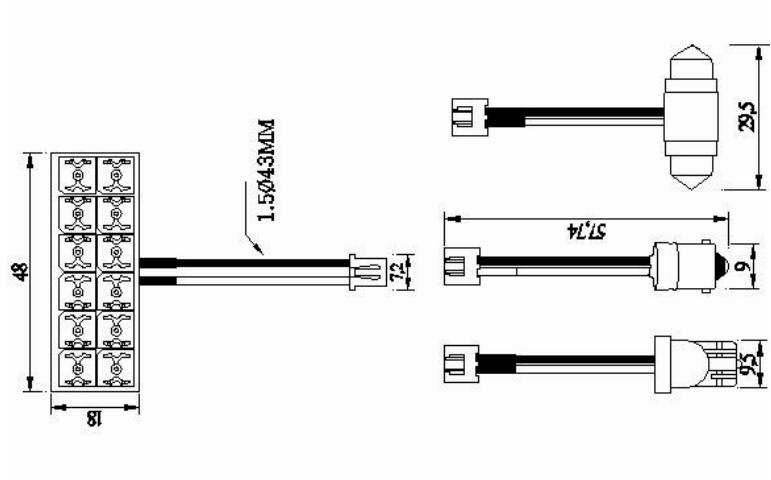
Doom – 12 SLED (10x31, BA9s, Wedge base)
